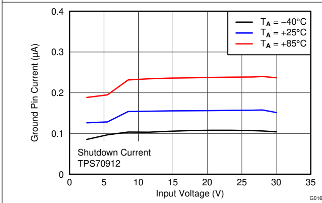
Fig 6-15. GND Current vs V_{IN} and Temperature
