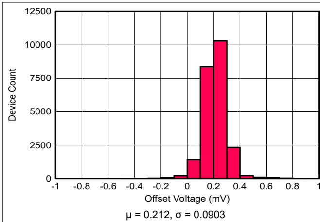
5-25. Voltage Offset Distribution
