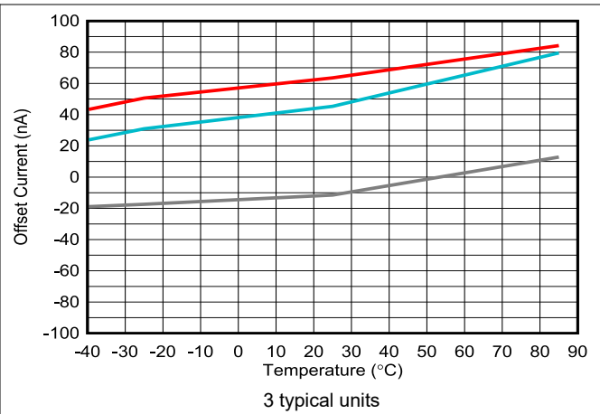
5-26. Input Offset Current vs Ambient Temperature
