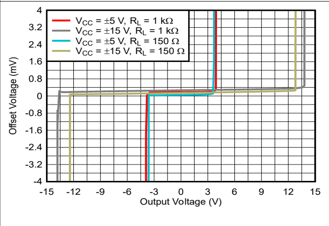
5-28. Offset Voltage vs Output Voltage
