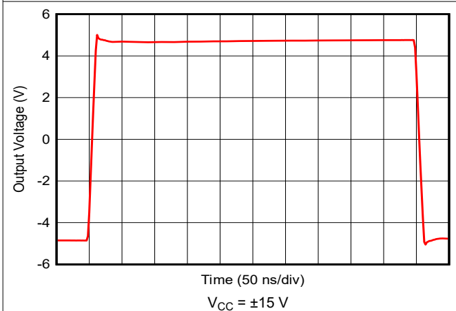
Figure 5-23. 10-V Step Response
