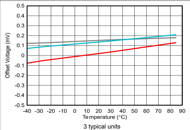
Figure 5-24. Input Offset Voltage vs Ambient Temperature
