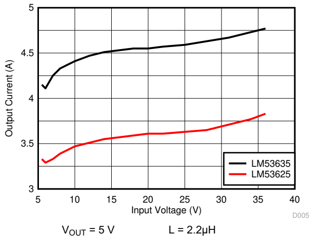
9-15. Output Current Level Limit Before Overcurrent Protection
