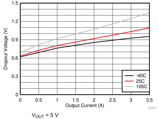
9-12. Dropout for \geq 1.85 MHz
