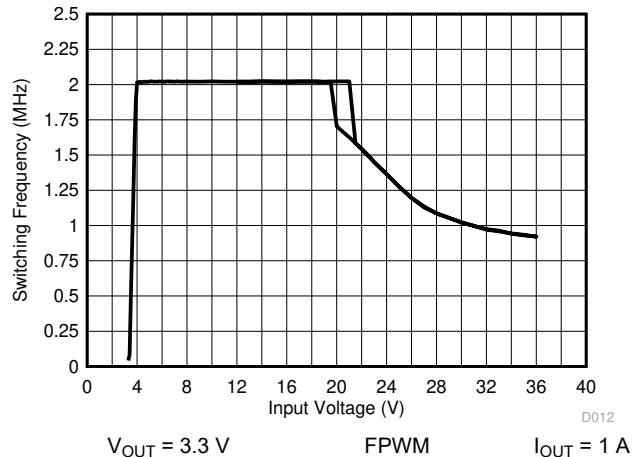
9-28. Switching Frequency vs Input Voltage
