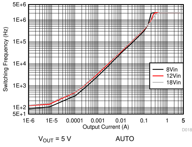
9-13. Switching Frequency vs Load Current
