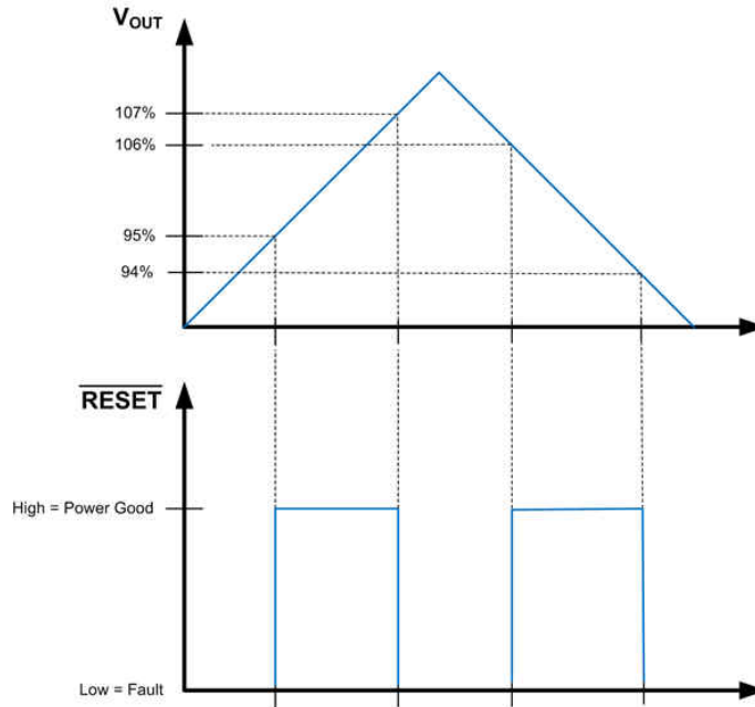
Figure 8-2. Static RESET Operation
