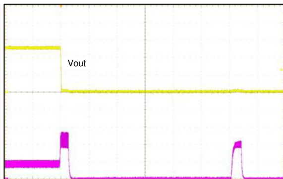
✎ 8-7. Hiccup Operation
