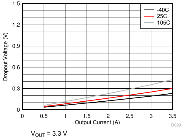
9-25. Dropout for -3\% Regulation
