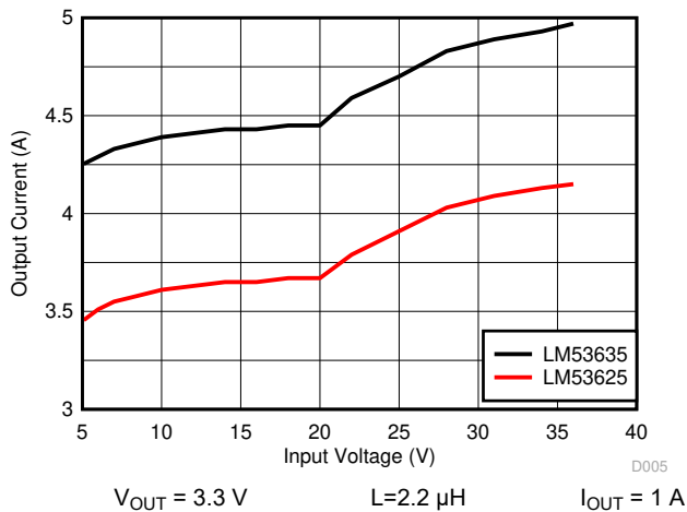
9-29. Output Current Level for Overcurrent Protection Trip
