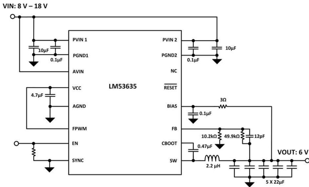
9-34. 6 V Output Power Supply
