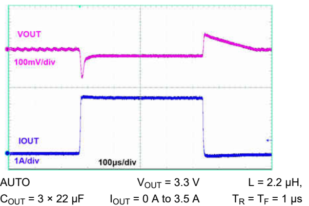
9-30. Load Transient
