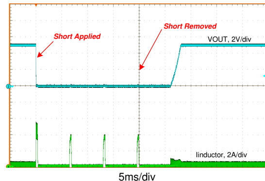
図 8-6. Short-Circuit Transient and Recovery
