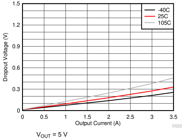
9-11. Dropout for -3% Regulation
