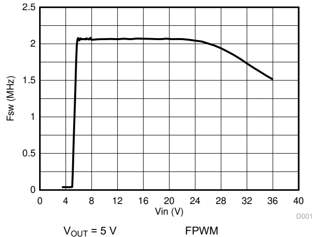
9-14. Switching Frequency vs Input Voltage
