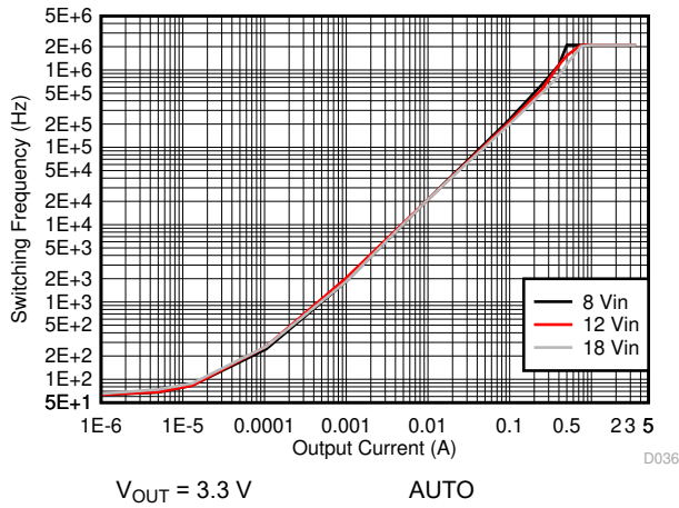
9-27. Switching Frequency vs Load Current
